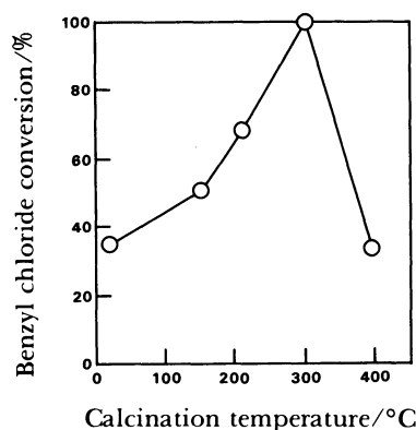
Fig. 3. Alkylation of toluene with benzyl chloride catalyzed by supported 12-molybdophosphoric acid (75 °C, 2 h). Heteropoly acid: 0.02 mmol; support: silica B (15 wt% loading); toluene: 100 mmol; benzyl chloride: 10 mmol.
